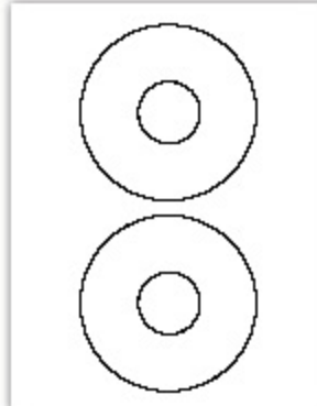
LW8-LIB-1519 Blank LW8-LIP-1519 Printed 2-up CD 4.625" diameter 1.625" inner circle diameter
